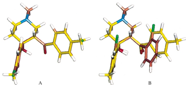
Figure 1. Superposition of the lowest energy conformations: (A) lead compound 3 (yellow), on analogue 12 (brown); (B) lead compound 3 (yellow) on analogue 16 (brown).
