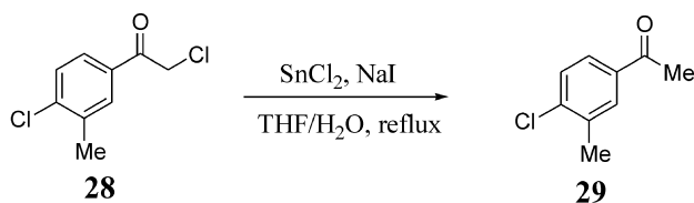
Scheme 1. Synthesis of intermediate 29 .
